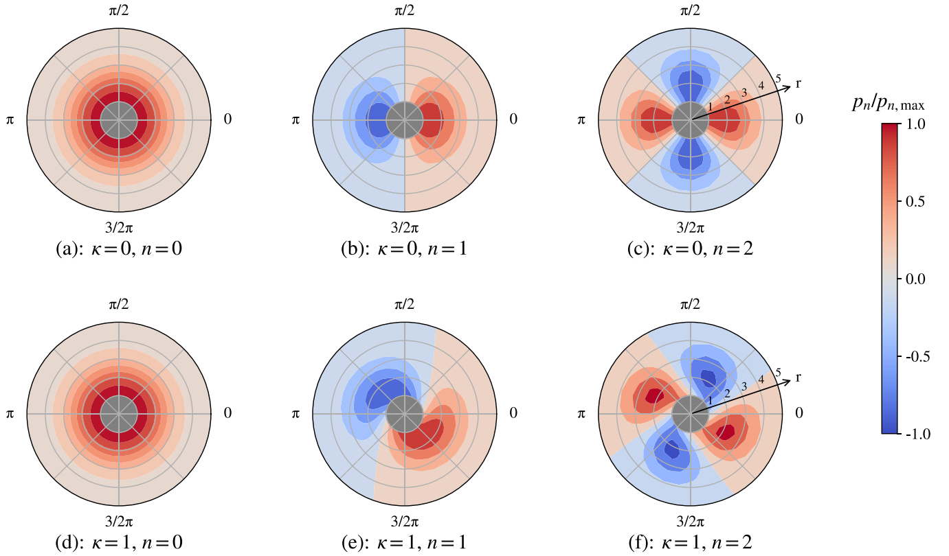
FIG. 1. Plots of the first three Fourier modes p_0 , p_1 , and p_2 of the relative PDF of interacting (odd-diffusive) particles p(r, \tau|r_0) = \Theta(r - 1) \sum_{n=0}^{\infty} p_n(r, \tau|r_0) at fixed time \tau = 1 . (a)–(c) Modes for normal particles ( \kappa = 0 ) and (d)–(f) for odd-diffusive particles ( \kappa = 1 ). The initial positions are chosen as (r_0, \varphi_0) = (1.01, 0) , i.e., the particles are placed 1.01 times their diameter along an arbitrarily defined x axis. The zeroth-order mode in (a) and (d) equals the mean positional PDF for the relative coordinate r [see Eq. (9)] which is unaffected by odd diffusion. The first order mode in (b) and (e), which corresponds to the (contracted) polarizational order PDF [see Eq. (10)], and the second order mode in (c) and (f), which corresponds to the (contracted) nematic order PDF [see Eq. (11)], as well as all higher order modes are affected by odd diffusion such that the modes are rotated in time compared to the \kappa = 0 case; see also Fig. 4. Note that the gray circle in the middle of each plot is due to the excluded volume condition \Theta(r - 1) of the hard-disk interaction of the particles.
