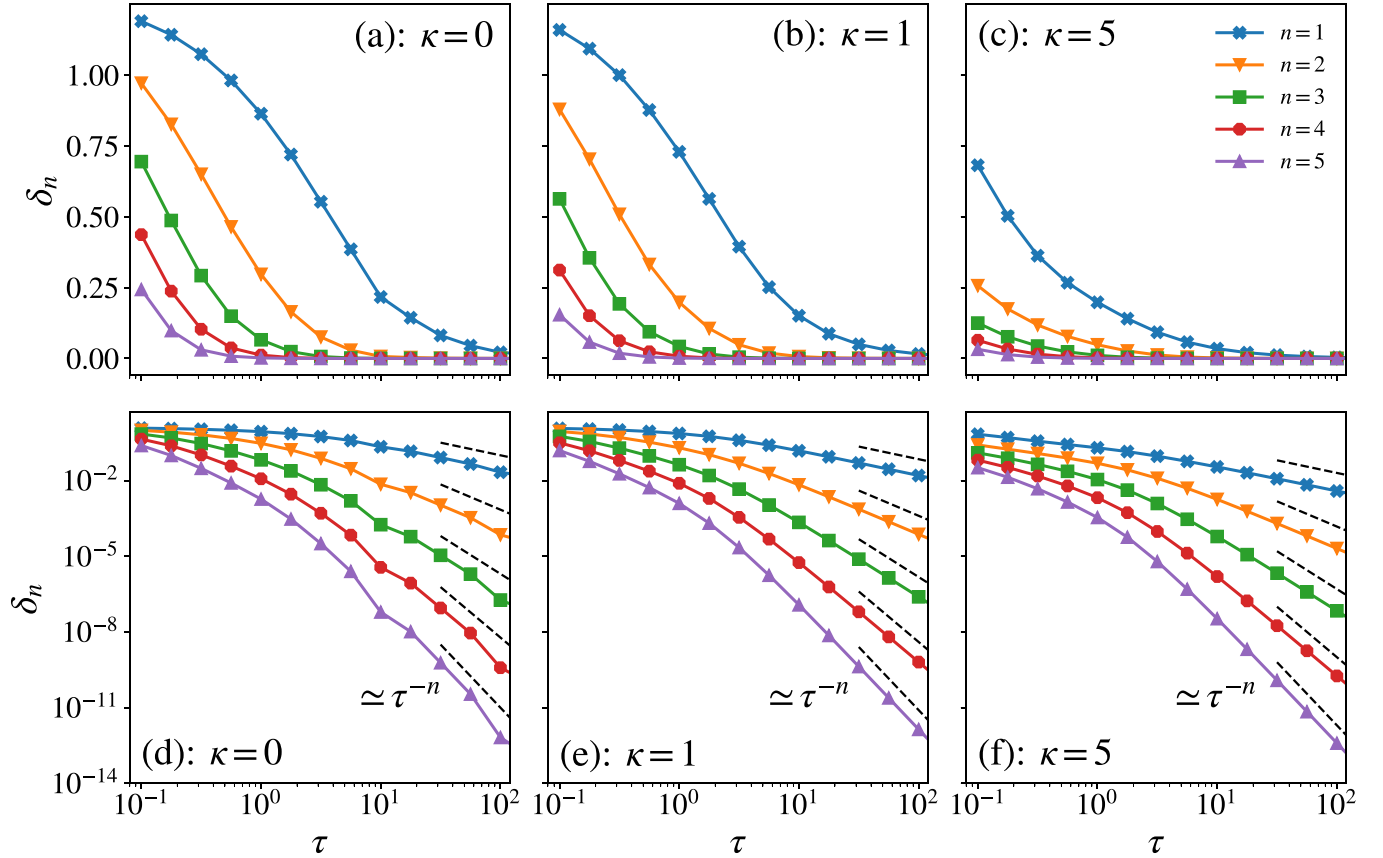
FIG. 2. Significance \delta_n(\tau) of a mode n as defined in Eq. (15), which measures the contribution of a Fourier mode of order n \geq 1 , p_n(\tau) , to the full relative PDF p(\tau) = \Theta(r-1) \sum_{n=0}^{\infty} p_n(\tau) as a function of time \tau for odd-diffusion parameter \kappa = 0, 1 and 5 in (a), (d); (b), (e); and (c), (f); respectively. We see that higher order modes are consecutively ordered in their contribution to p in time and become of comparable importance for \tau \rightarrow 0 as p(\tau) \rightarrow p(0) \propto \delta(\mathbf{x} - \mathbf{x}_0) . Comparing (a) with (c), we observe that \kappa > 0 shifts the characteristic decay to shorter times. Thus, for dynamics where one is not interested in the \tau \rightarrow 0 limit, one can truncate the Taylor expansion at finite n . (d)–(f) Algebraic decay of \delta_n(\tau) \simeq \tau^{-n} for \tau \rightarrow \infty , independently of \kappa .
