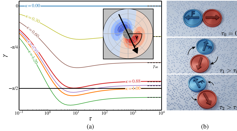
FIG. 4. (a) Angle \gamma(\tau) between the polarization mode \sigma(r=1, \tau|r_0=1) , Eq. (10), and its initial direction as function of time \tau for different odd-diffusion parameters \kappa ; see Eq. (19) and the inset. The polarization mode constitutes the vectorial mode of the relative PDF p(\tau) for interacting particles and represents relative particle rearrangements. In a normal system ( \kappa=0 ), \gamma(\tau)=0 and is constant in time, whereas it develops an extremum \gamma_{\text{ext}} different from its asymptotic steady state value \gamma_\infty = -\arctan(2\kappa/(1-\kappa^2)) (dashed lines) for \kappa \neq 0 in time. We observe that |\gamma_{\text{ext}}| > |\gamma_\infty| , indicating that particles on average rotate further in time than they finally relax to. Specifically for \kappa \in (0.88, 1.0) , \gamma_{\text{ext}} < -\pi/2 , but \gamma_\infty > -\pi/2 which quantitatively aligns with the oscillating FACF previously observed for this regime [9]. (b) The sketch qualitatively illustrates the scenario, that odd-diffusive particles with 0.88 < \kappa < 1 collide at \tau_0 with each other along the (arbitrary) x axis and rotate for \tau_1 > \tau_0 to \gamma_{\text{ext}} < -\pi/2 , and eventually relax at \tau_2 > \tau_1 to \gamma_\infty > -\pi/2 .
