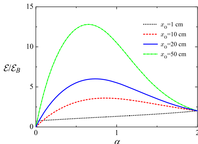
Figure 6. Search efficiency as function of the stable index \alpha for fixed x_0 , K_\alpha = 1 \text{ cm}^\alpha \text{ s}^{-1} , K_2 = 1 \text{ cm}^2 \text{ s}^{-1} .
