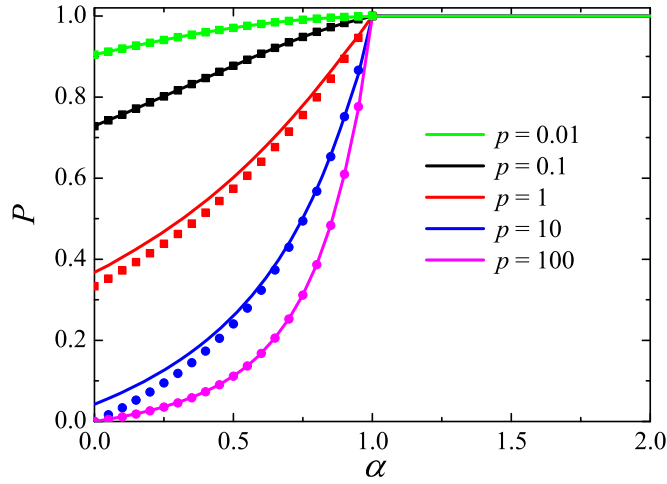
Figure 3. Search reliability P as function of the Lévy stable exponent \alpha for various values of p , equation (12). The continuous curves are obtained by numerical computation of equation (11). The squares for the cases p = 0.01 (green), p = 0.1 (black) and p = 1 (red) are obtained from the approximation (17) for small p . The circles of corresponding colour are plotted from the approximate expression (19) for large p .
