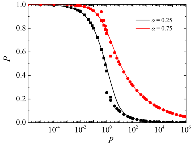
Figure 4. Search reliability as a function of the parameter p = x_0^{2-\alpha} K_\alpha / K_B for various stable indices \alpha . Continuous lines were obtained from numerical solution of equation (11). The squares show the analytical approximation (17) for small p . The circles are plotted from the approximate expression (19) for large p .
