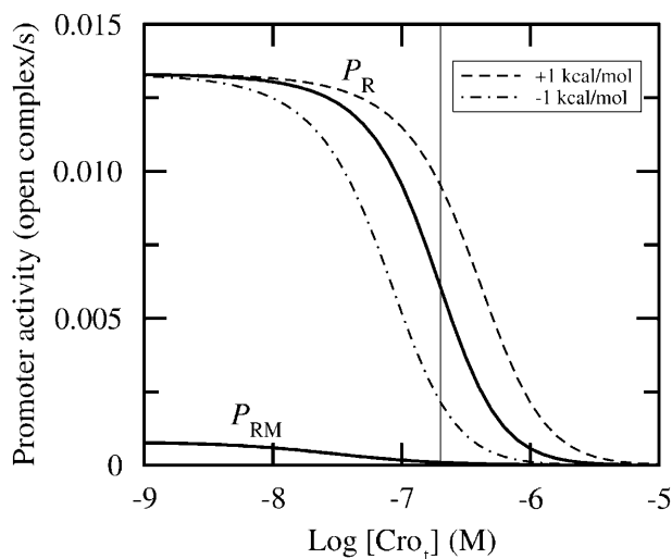
FIGURE 6 Promoter activity versus total Cro concentration for [CI] \approx 0 (fully drawn line). Dashed lines correspond to \Delta G_{1'} perturbed \pm 1 kcal/mol. Perturbations have negligible impact on the activity at P_{RM} . Thin vertical line indicates 200 nM. Abscissa is drawn on logarithmic (decadic) scale.
