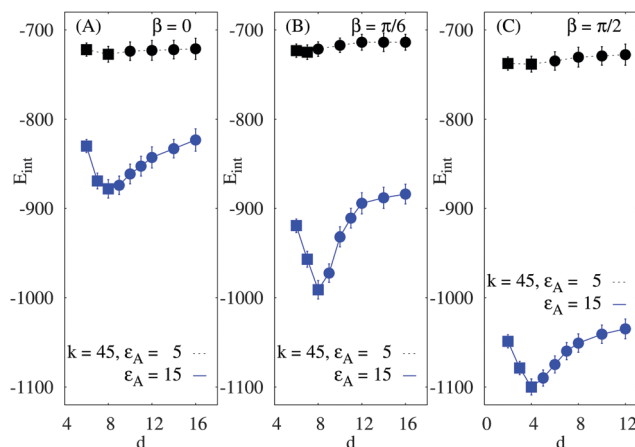
Fig. 8 Interaction energy E_{\text{int}}(d) of substrate-adhered rods versus inter-axial distance d , plotted for \beta = 0, \pi/6 , and \pi/2 (from left to right). Other parameters are indicated in the plots. The circles and squares designate the regions of attraction and repulsion, respectively. The error bars are shown.
