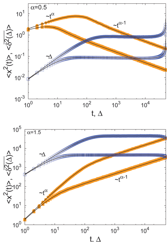
Fig. 19 MSD \langle x^2(t) \rangle (orange symbols) and time averaged MSD \langle \overline{\delta^2(\Delta)} \rangle (blue symbols) of SBM with \alpha = 0.5 (top) and \alpha = 1.5 (bottom). In each case we consider the potential strengths \omega^2 = 0.01 (circles) and \omega^2 = 0.1 (squares). The full lines represent eqn (83) and the numerical evaluation of the exact results for the time averaged MSD. 189 The convergence of the corresponding ensemble and time averages at \Delta = t = 10^5 can be shown numerically, in analogy to Fig. 18 for the unconfined motion.
