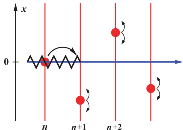
Fig. 14 Sketch of the crack propagation model discussed in the text. The tip of the crack (black zig-zag line) propagates from site n to n + 1 when the vacancy represented by the red circle diffuses to the origin ( x = 0 ) at point n .
