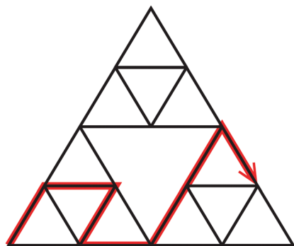
Fig. 24 A random walk on part of a Sierpiński gasket. Each time the walker wants to reach a sector of the gasket across one of the larger holes, it needs to traverse a narrow causeway.
