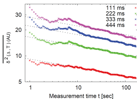
Figure 8. Time-averaged MSD for the motion of potassium channels in plasma membranes plotted as a function of measurement time at given lag times \Delta = 111, 222, 333, and 444 ms. The time dependence shows that the process ages. The straight dashed lines represent fits with slope \alpha - 1 = -0.10 , while the particle motion is represented with a CTRW. Reproduced with permission from ref 53. Copyright 2011 National Academy of Sciences.
