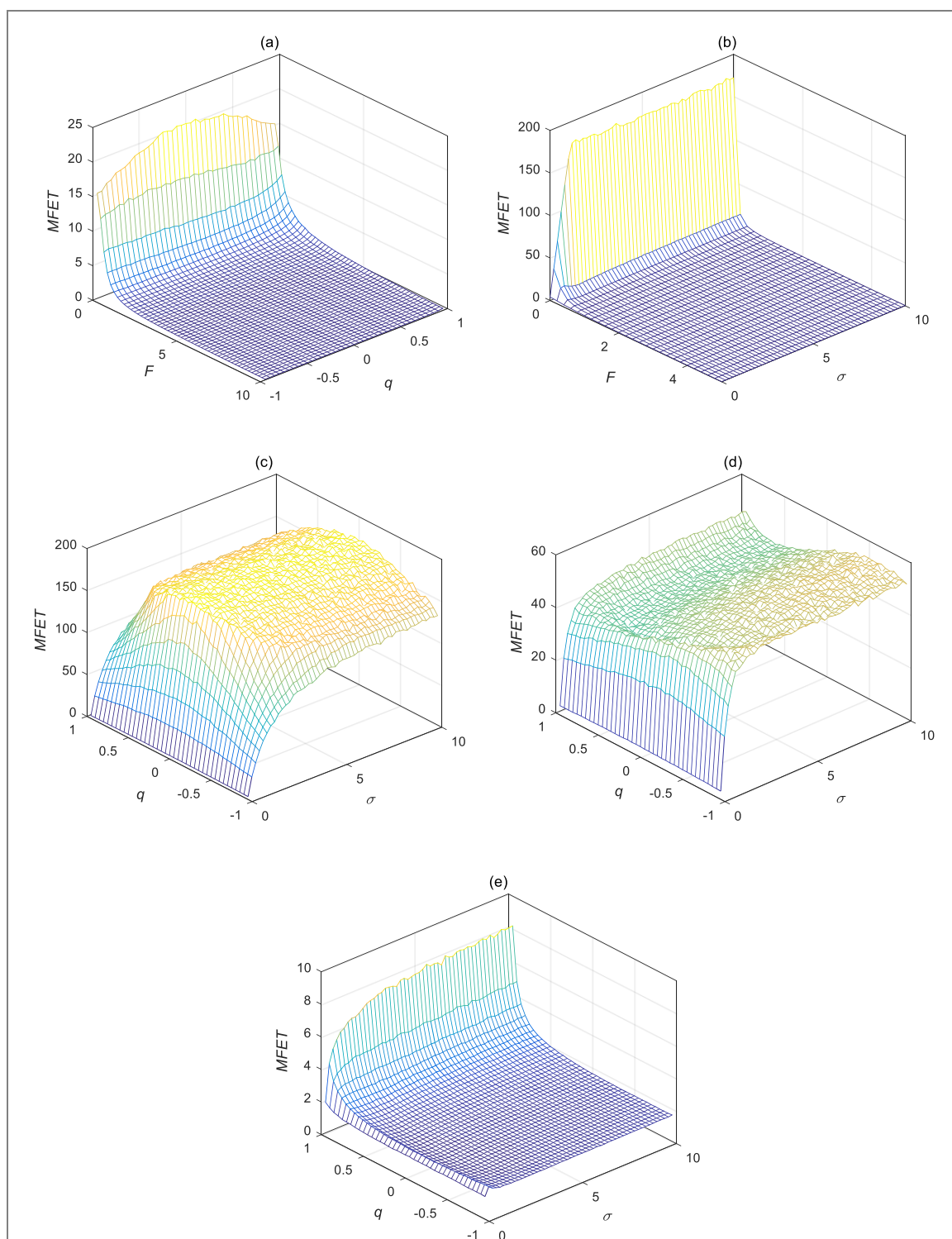
Figure A5. MFETs for D_d(x, y) in the isothermal interpretation. (a) \sigma = 0.1 when F = 0 , the MFET decreases with |q| . For large F , the MFET will increase with q . (b) q = 0 . For F = 0 , the MFET will first increase fast with \sigma , and then it will remain almost constant. For small F \neq 0 , the MFET will first increase, then decrease and then increase, resulting in minimal MFET at \sigma = 1 . This is consistent with figure A3. For large F , the MFET will first decrease and then increase. (c) F = 0 . The MFET is much smaller for a small \sigma than for a large \sigma . For fixed q , with increasing \sigma the MFET first increases fast and then levels off. (d) F = 0.1 . Due to the interactions with the noise-induced drift, the variation of MFET with respect to q and \sigma is complex. It will further change with increasing F . However, we see that a small change for F will cause a large reduction for the MFET. (e) F = 1 . With a larger F than that of (d), the MFET becomes totally different. For large q , the MFET increases almost monotonically with \sigma , however, for a q > 0.9 , the MFET first increases, then decreases and increases. Finally, for a fixed \sigma , the MFET will decrease with decreasing q .
