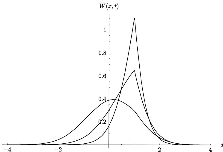
Fig. 17. Pdf W(x, t) , Eq. (119), of the fractional Ornstein-Uhlenbeck process, for the anomalous diffusion exponent \alpha = 1/2 . The initial value is chosen to be W_0(x) = \delta(x - 1) . The maximum clearly slides towards the origin, acquiring an inversion symmetric shape. The curves are drawn for the times t = 0.02, 0.2 , and 20 , employing the integral relation with the Brownian solution. Note the distinct cusps around the initial position. Compare Fig. 18.
