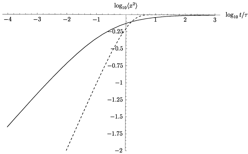
Fig. 20. Mean squared displacement for the fractional ( \alpha = 1/2 , full line) and normal (dashed) Ornstein-Uhlenbeck process. The normal process shows the typical proportionality to t for small times, and approaches the saturation value much faster than its subdiffusive analogue which starts off with the t^{1/2} behaviour and approaches the thermal equilibrium value by a power-law, compare Eq. (122).
